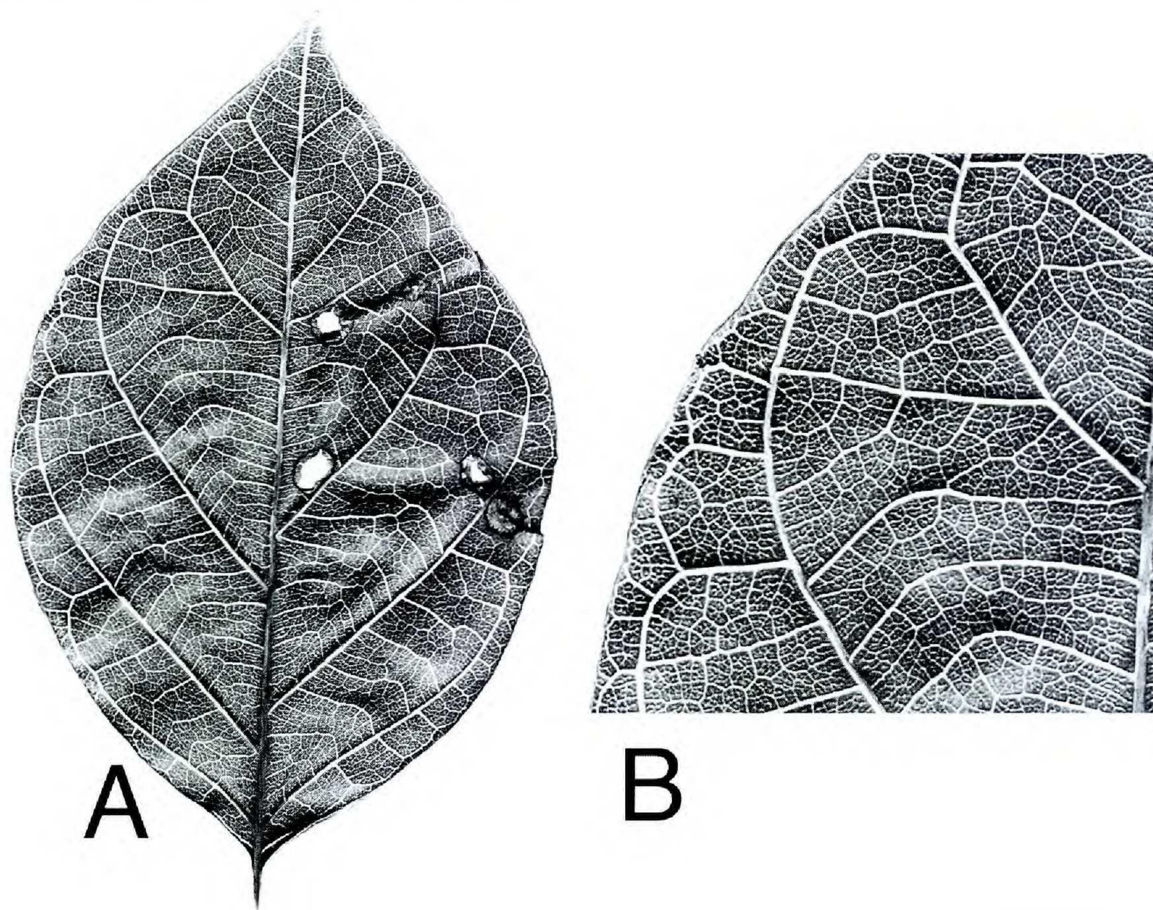
FIG. 2. A, typical leaf of Campomanesia guabiroba showing its venation pattern (blade 9 cm long). B, magnified view of portion of same leaf showing detail of venation (Landrum 2490, ASU).
